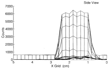
Figure 4.12 End and side views of the monostatic acoustic pulse for 1.3 MHz and wire of radius 40 microns.
